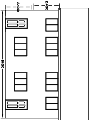
Front Elevation
