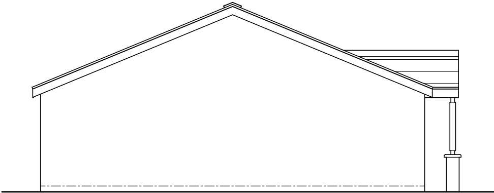
PROPOSED SIDE (EAST) ELEVATION 1:100 scale
