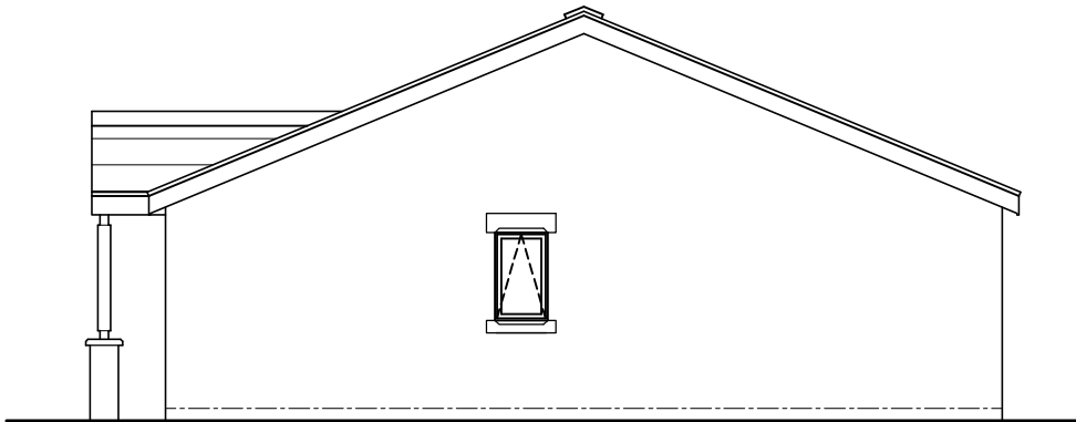
PROPOSED SIDE (WEST) ELEVATION 1:100 scale
