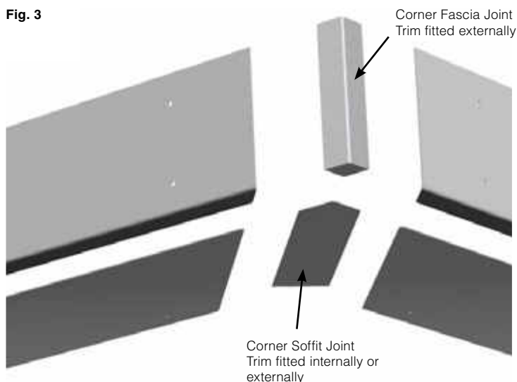
Jointing - Corner Detail
