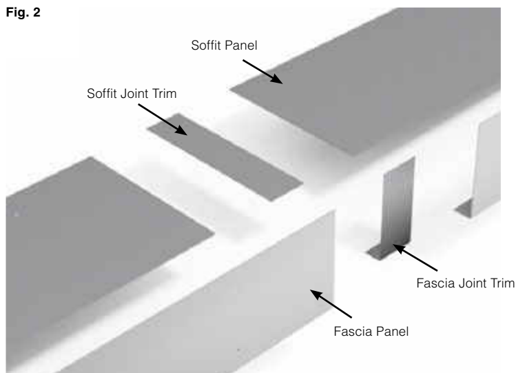
Jointing - Straight sections
