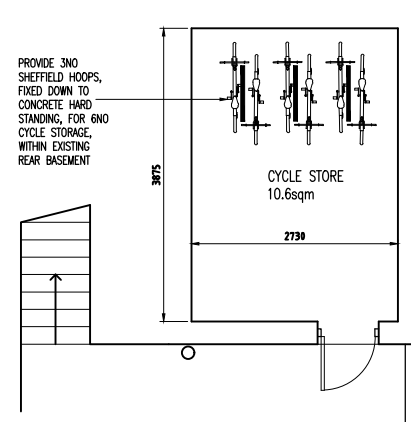
PROPOSED BASEMENT FLOOR PLAN 1:100 @ A3
