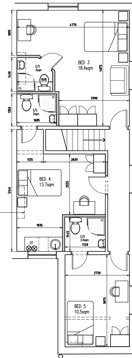
PROPOSED FIRST FLOOR PLAN 1:100 @ A3
