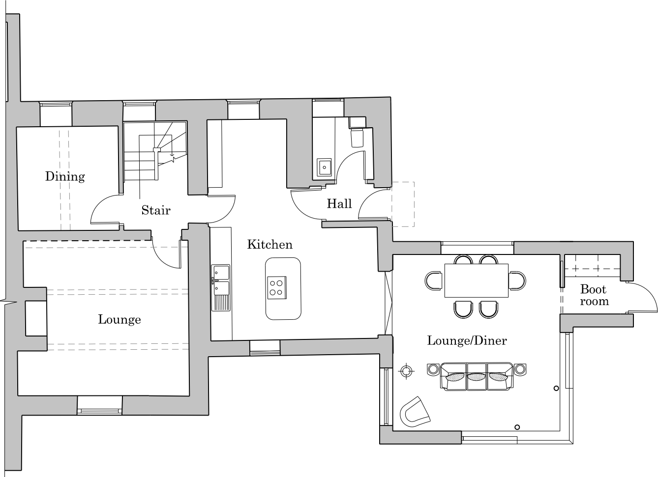
Ground Floor
