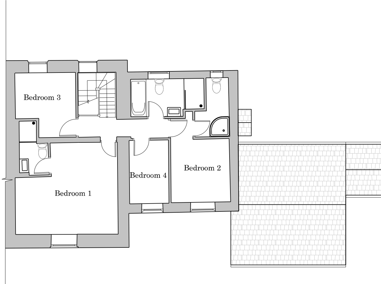
First Floor
