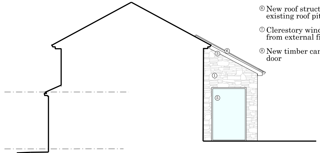
Elevation D
