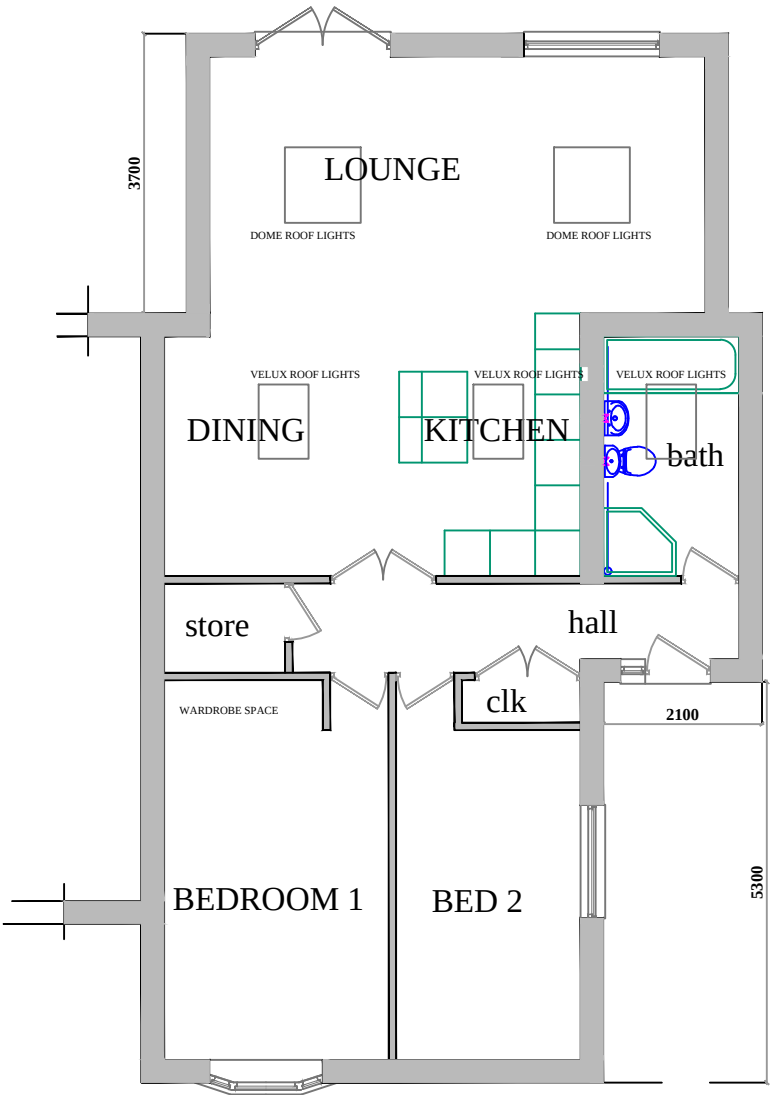
PROPOSED PLAN
