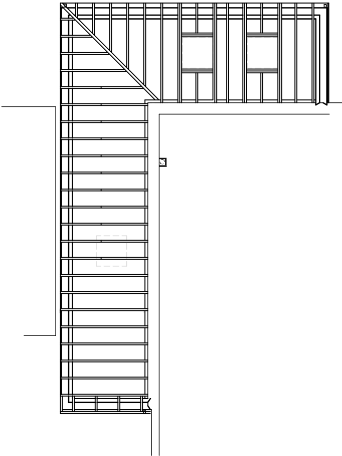
PROPOSED ROOF STRUCTURE PLAN 1:100
