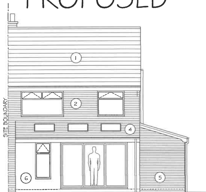
PROPOSED NORTH WEST ELEVATION 1:100
