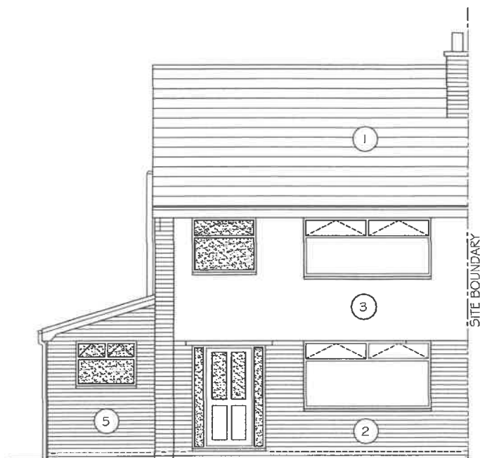
PROPOSED SOUTH EAST ELEVATION 1:100
