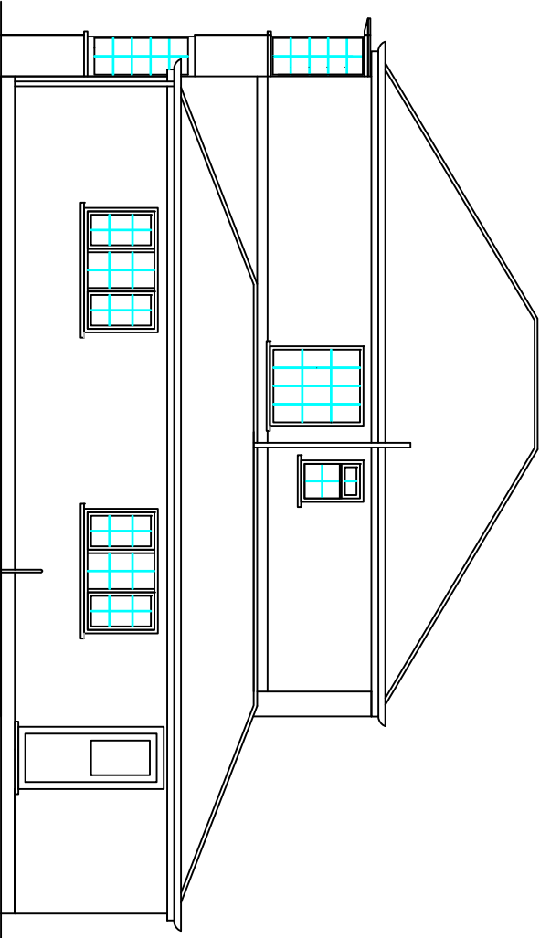
Side Elevation
