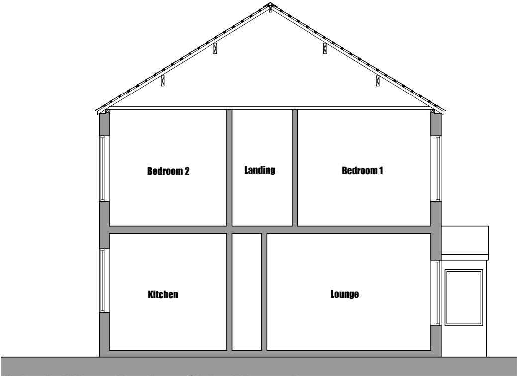
South West Facing Side Elevation
