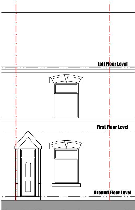
North West Facing Front Elevation
