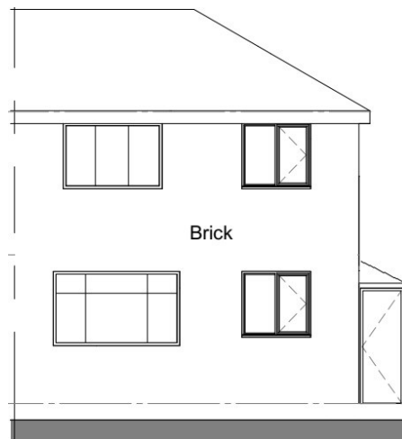
Rear elevation
