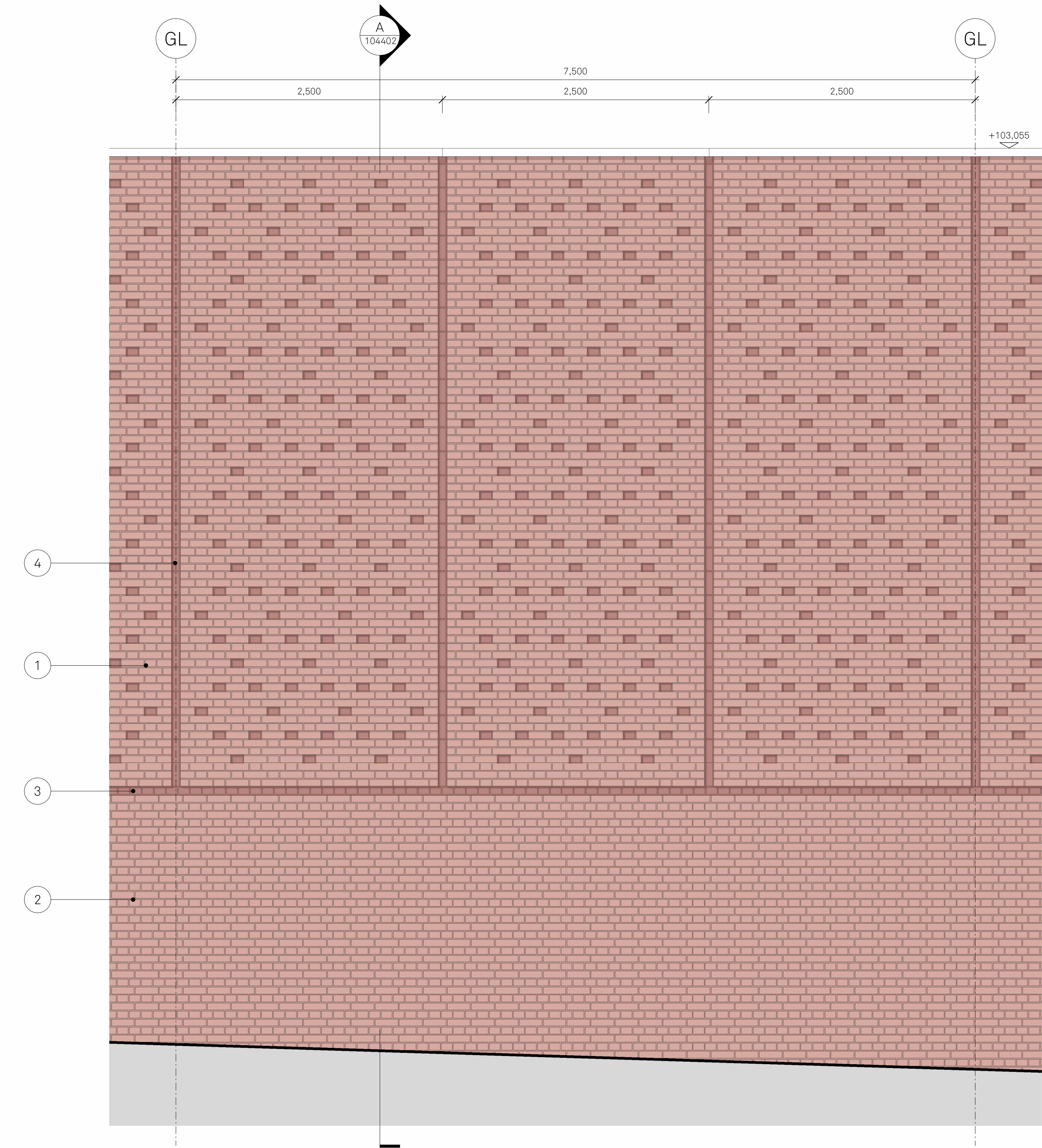
1 DETAIL ELEVATION HIGHFIELD ROAD ELEVATION
