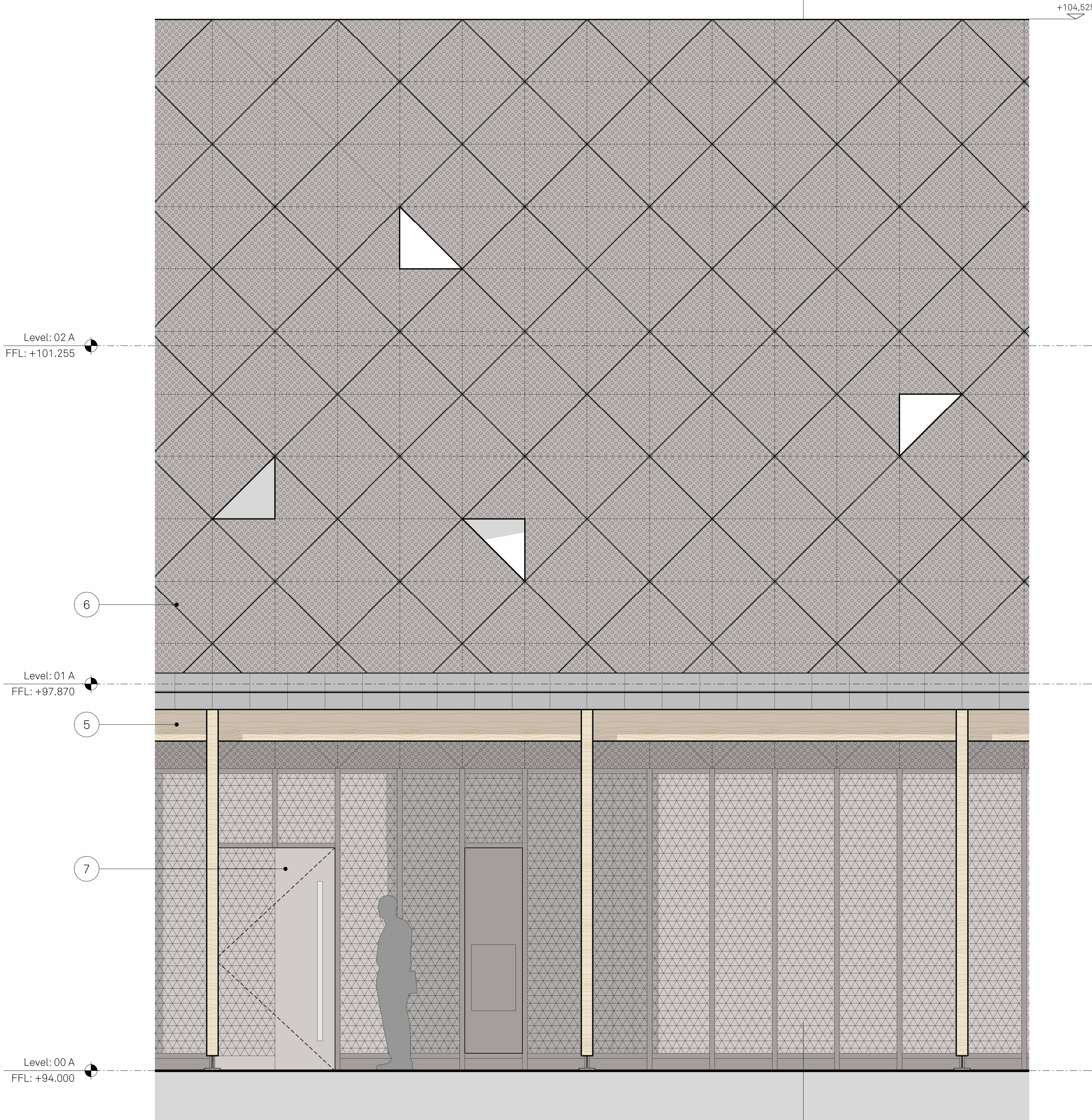
1 DETAIL ELEVATION FAIRFAX ROAD
