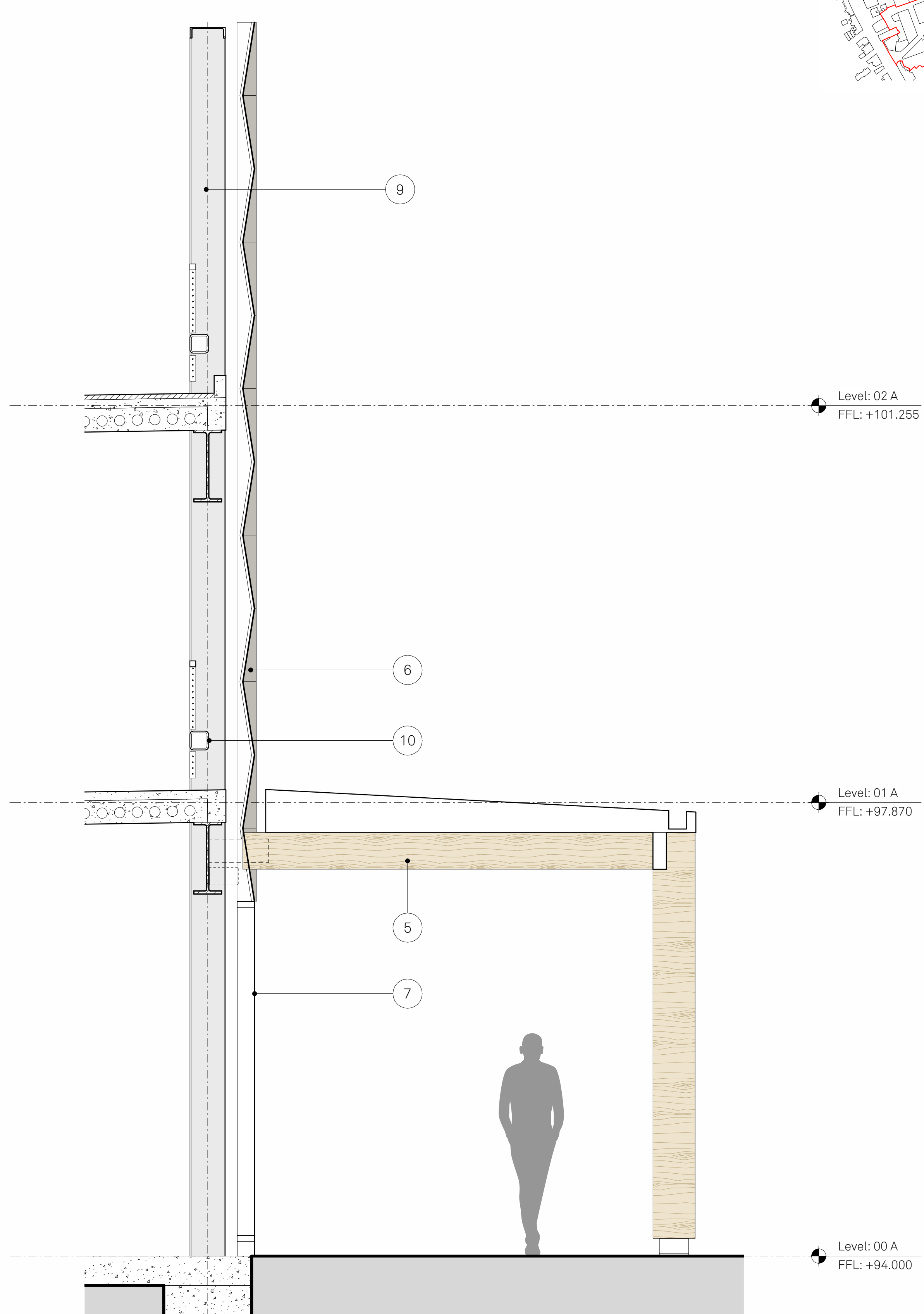
A SECTION FAIRFAX ROAD
