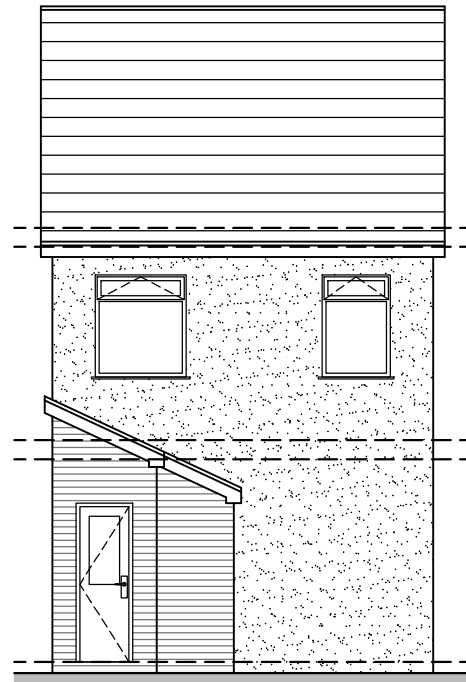
REAR ELEVATION
