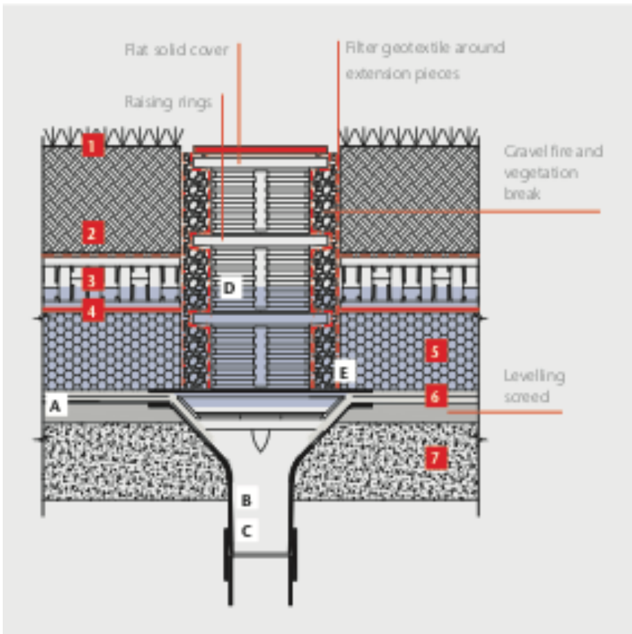
Sectional Detail - Aco Blue/Green Roof System - Plan Ref R.01.G & R.01.B
