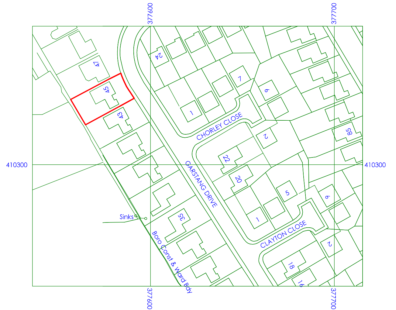
LOCATION PLAN 1:1250 SCALE NORTH^
