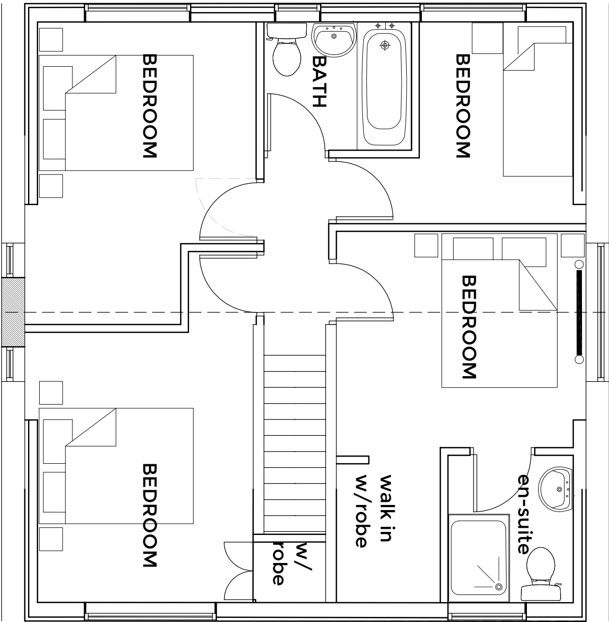
PROPOSED FIRST FLOOR/LOFT PLAN 1:50
