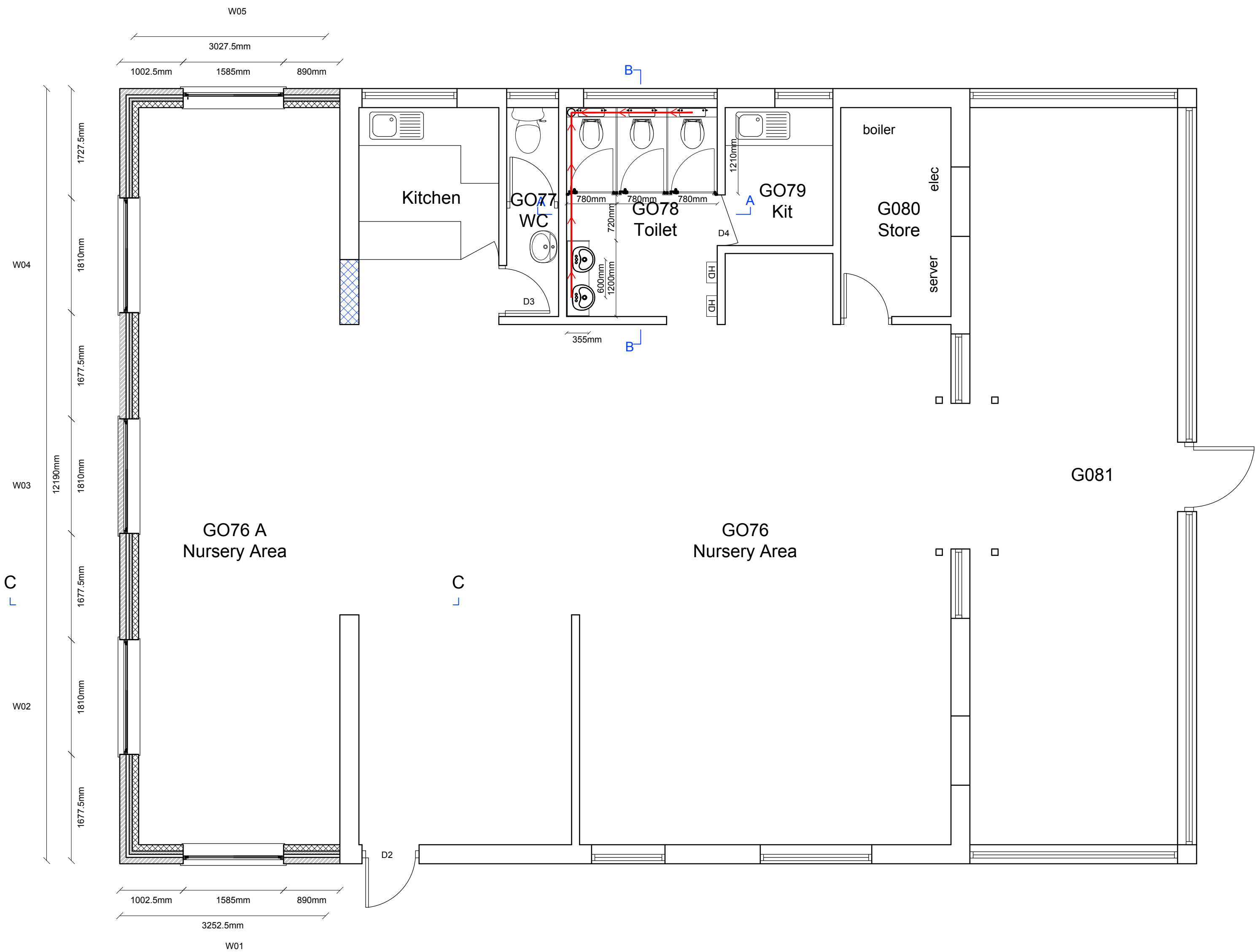
Proposed Layout Plan 1:50 @A1
