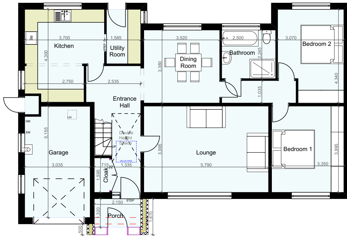
PROPOSED GA GROUND FLOOR PLAN
