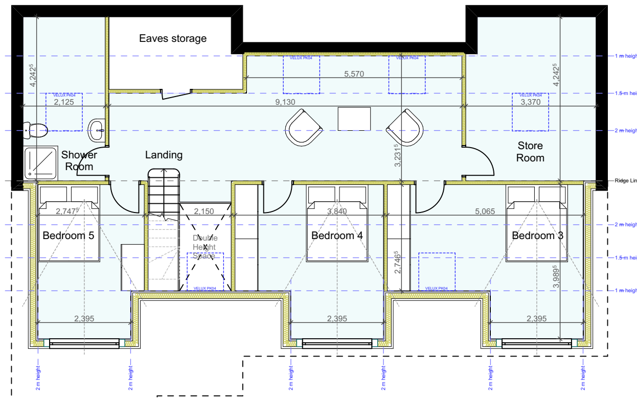
PROPOSED GA FIRST FLOOR PLAN
