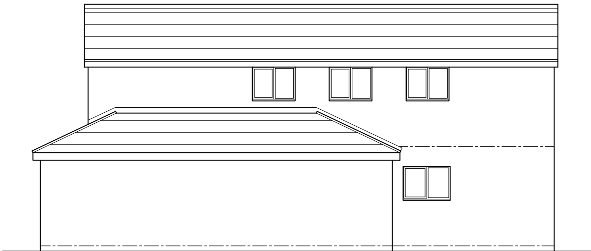
EXISTING SIDE/SOUTH EAST ELEVATION (1:100)
