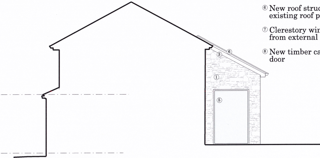
Elevation D
