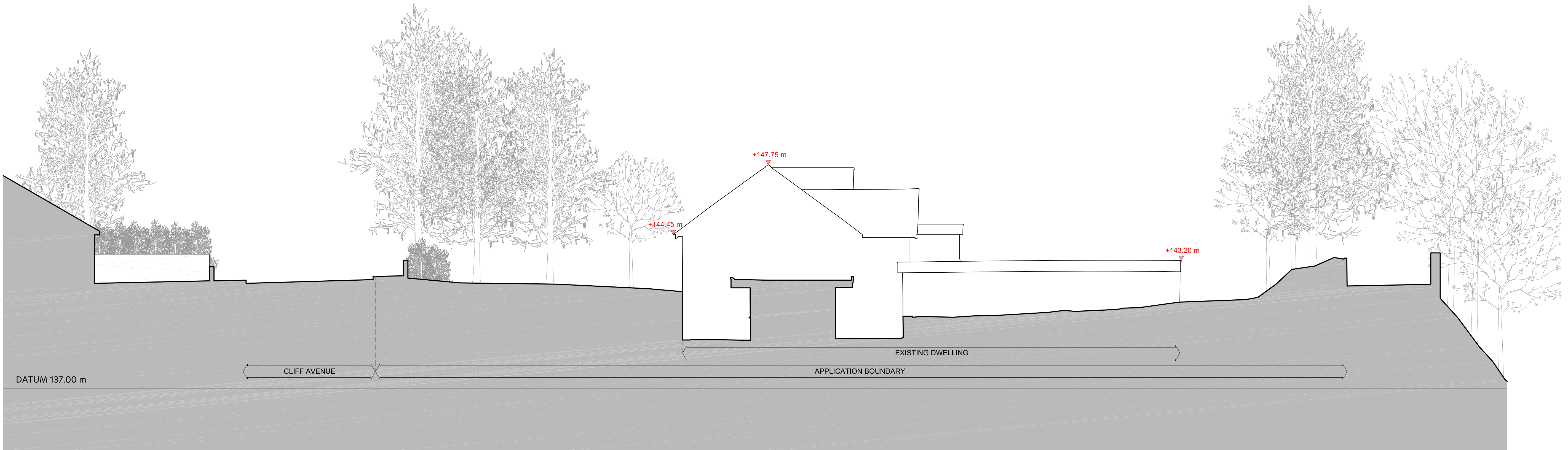
EXISTING SITE SECTION A-A (NORTH-SOUTH)
