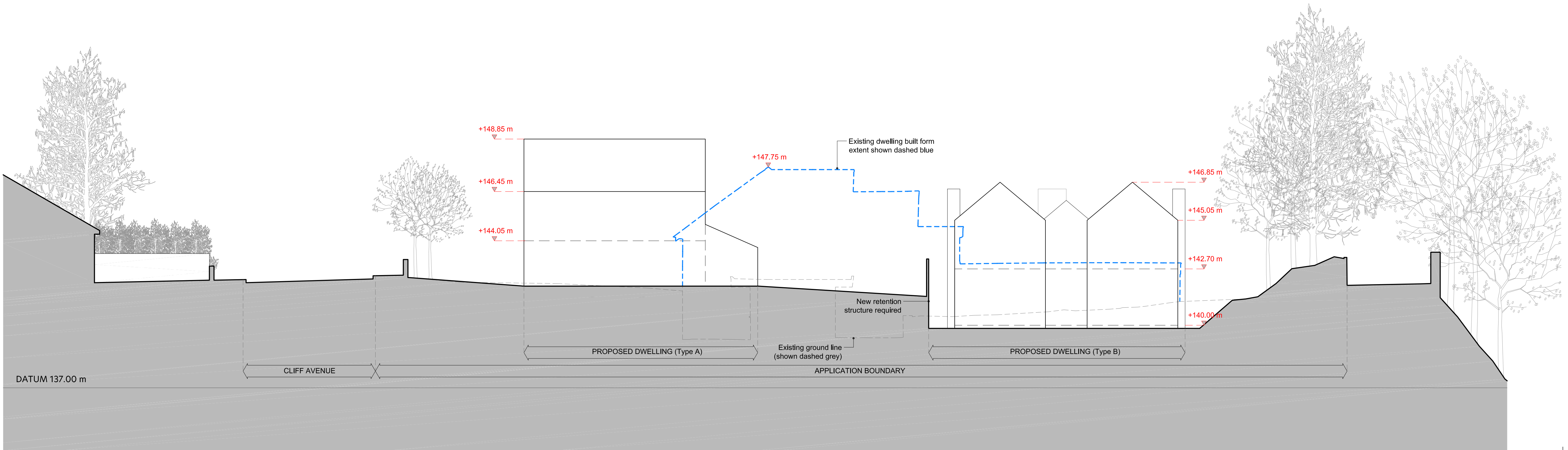
PROPOSED SITE SECTION A-A (NORTH-SOUTH)
