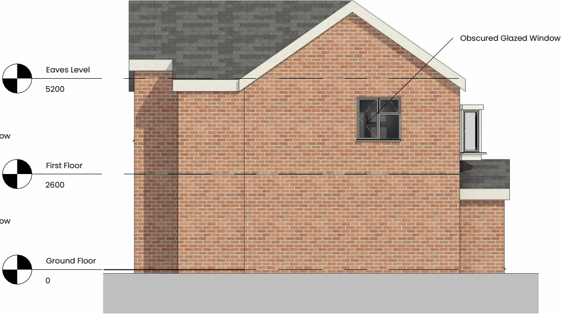
4 Proposed Side Elevation B 1 : 100
