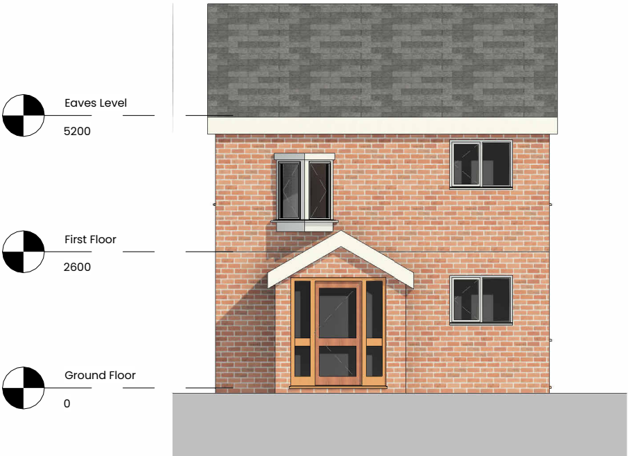
2 Proposed Rear Elevation 1 : 100
