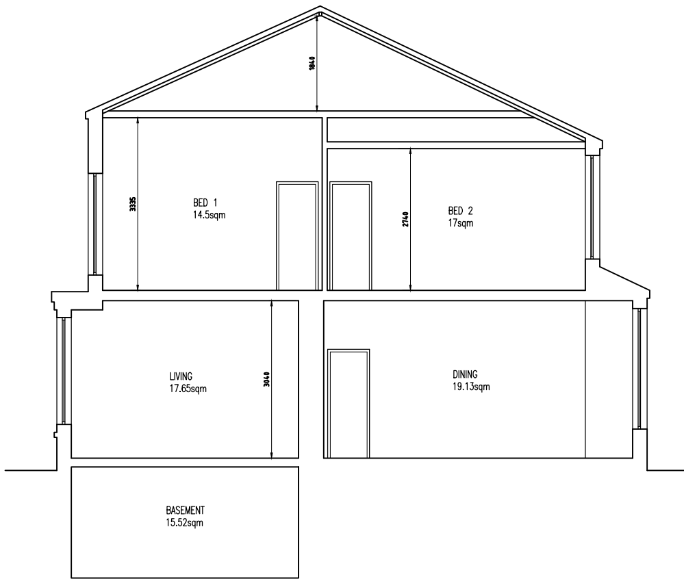
EXISTING SECTION 1:100
