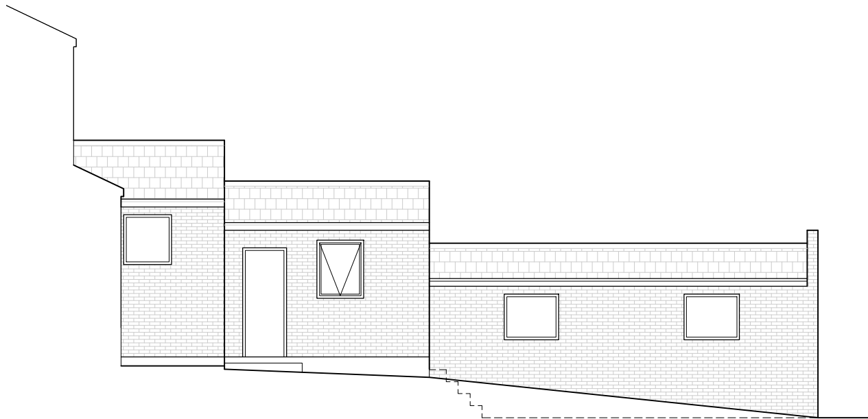
EXISTING REAR SIDE ELEVATION (EAST FACING) 1:100
