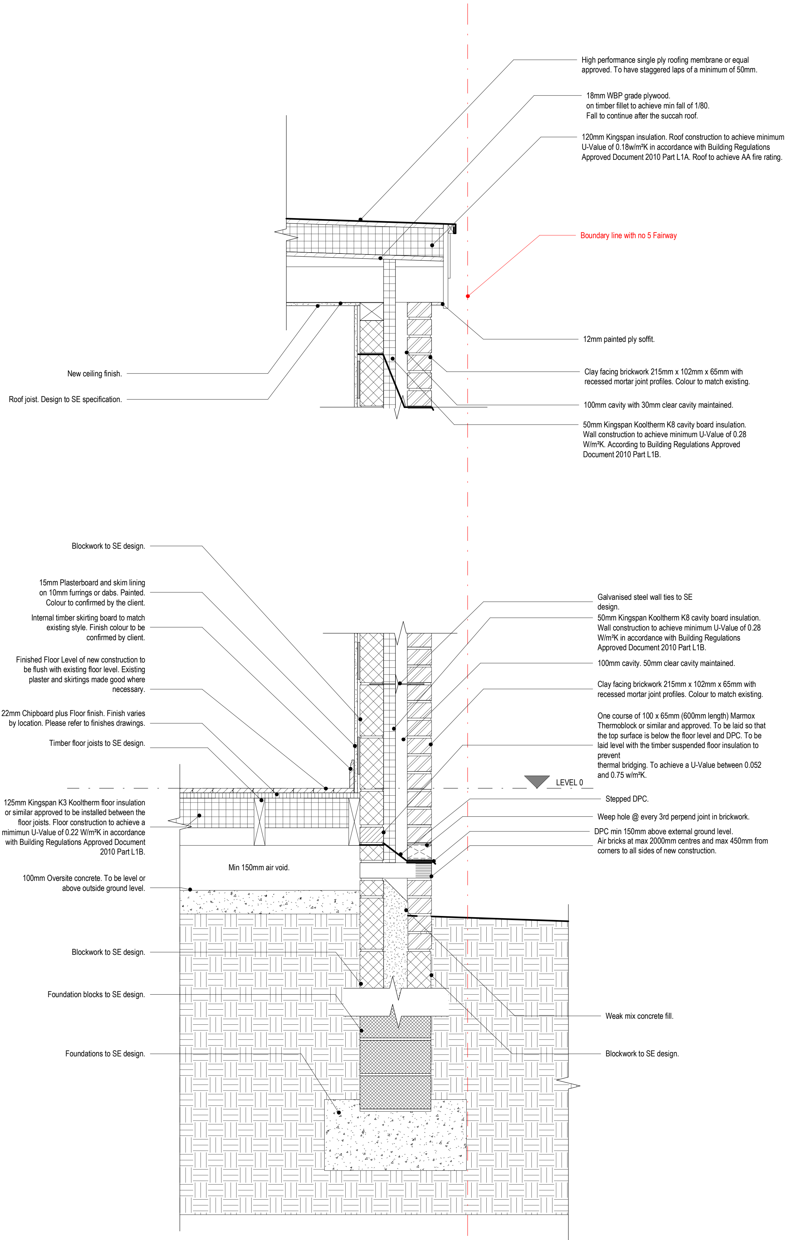
1 Boundary wall detail 1 : 10
