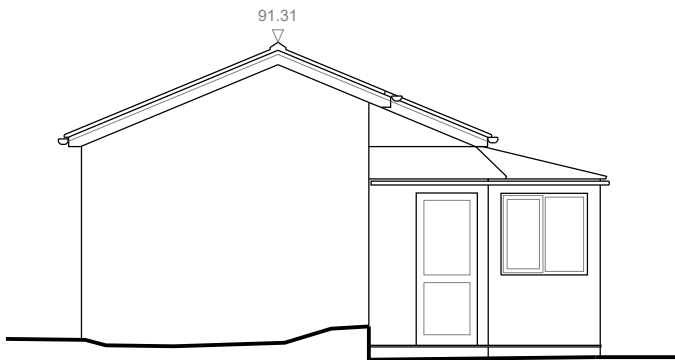
PROPOSED LEFT SIDE ELEVATION
