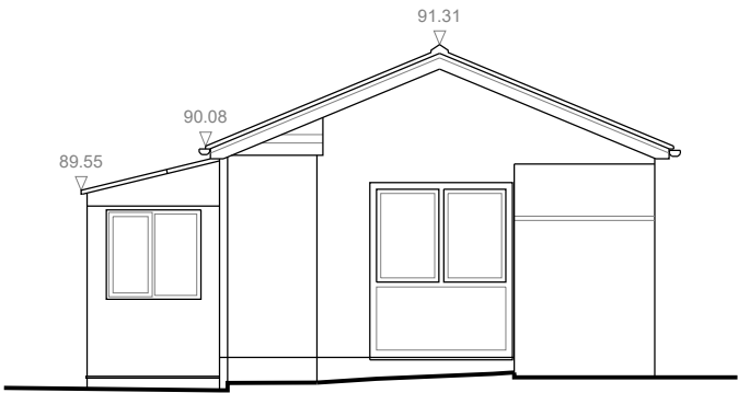
PROPOSED RIGHT SIDE ELEVATION
