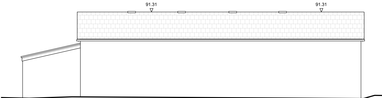
PROPOSED REAR ELEVATION
