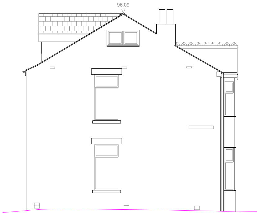
PROPOSED LEFT SIDE ELEVATION
