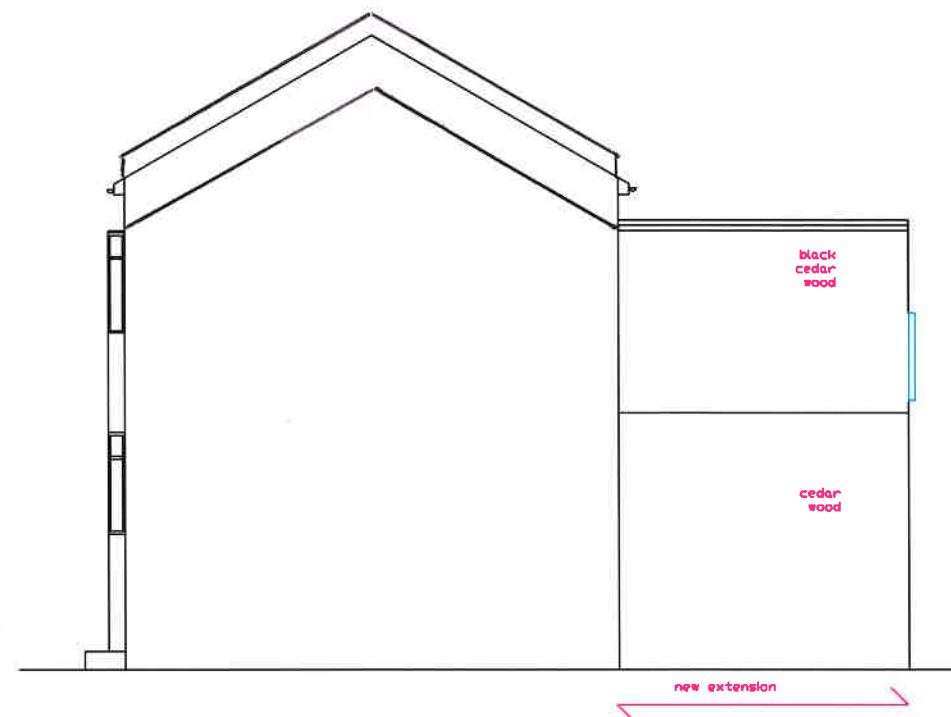
PROPOSED SIDE VIEW B 1:100
