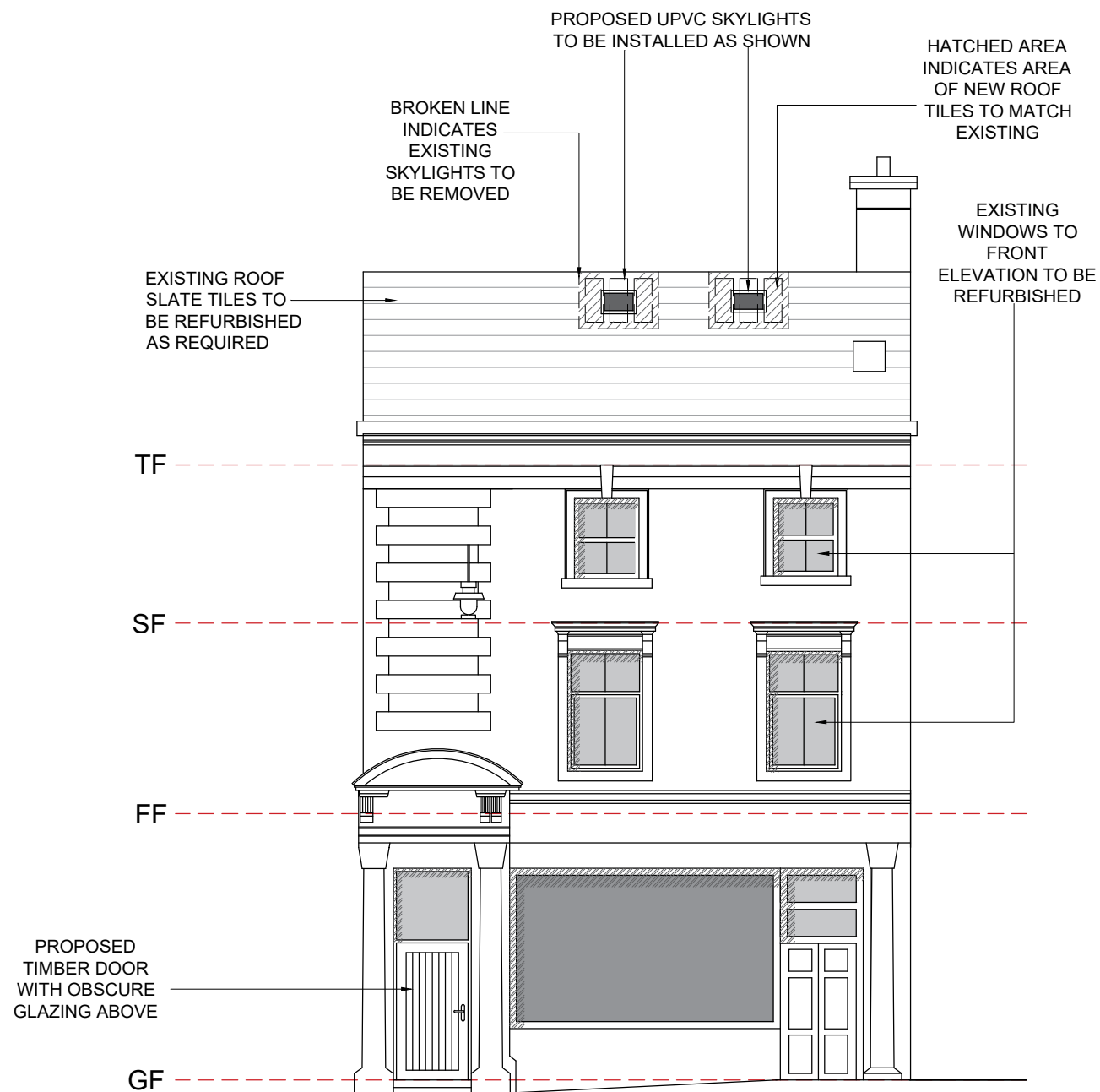
FRONT ELEVATION
