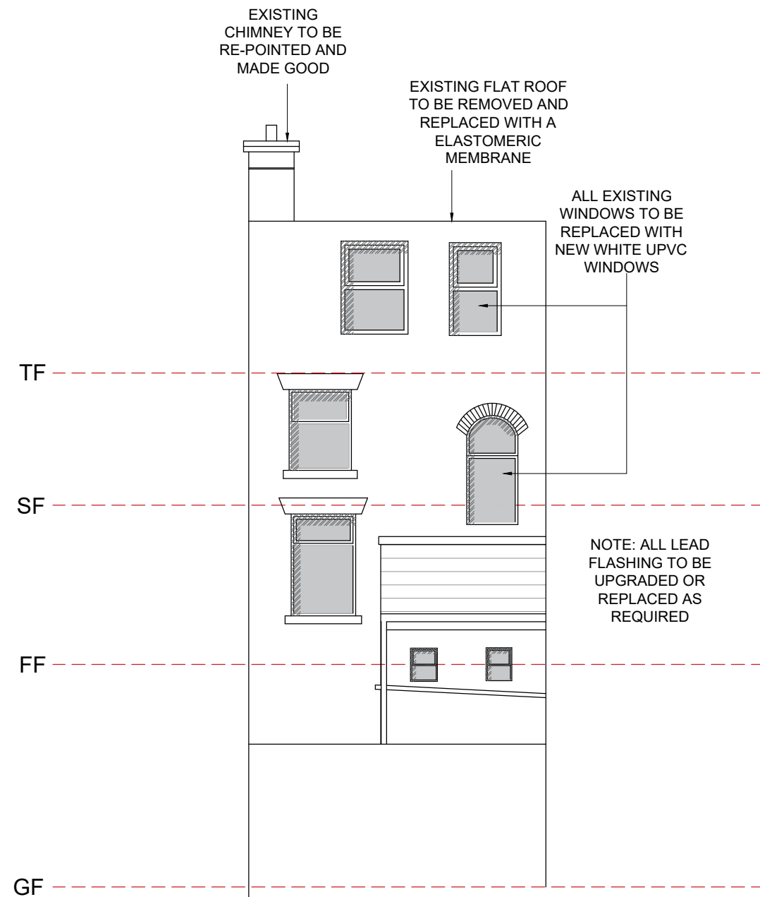
REAR ELEVATION
