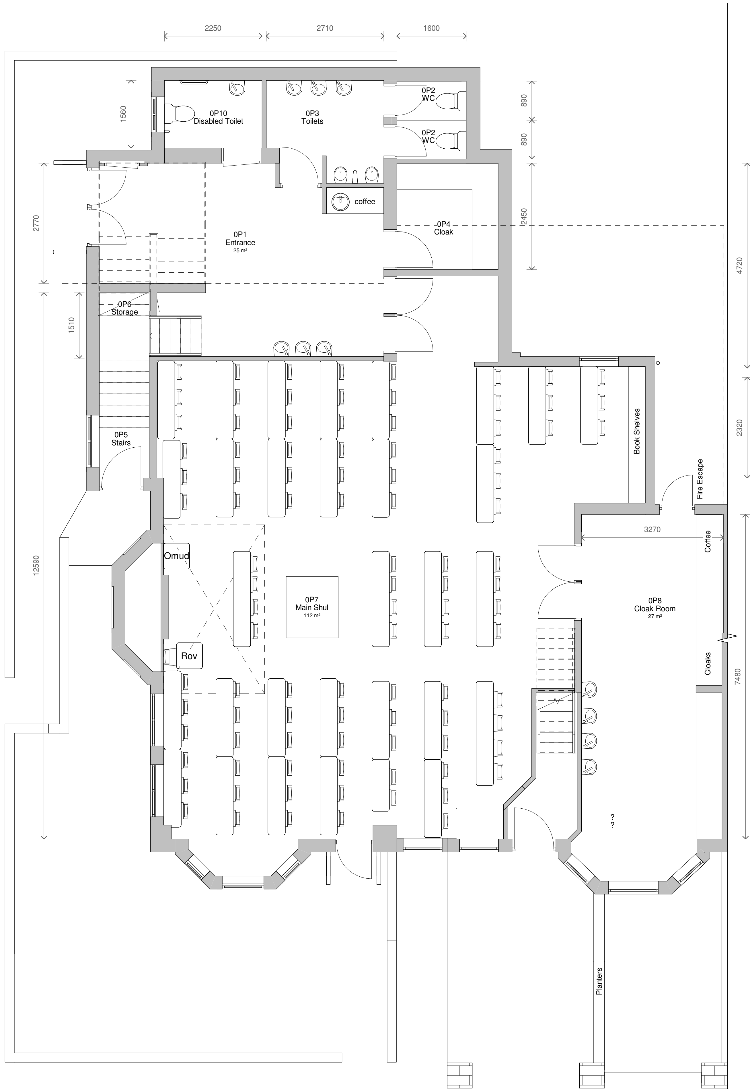
1 Level 0 - 72-74 Proposed 1 : 50
