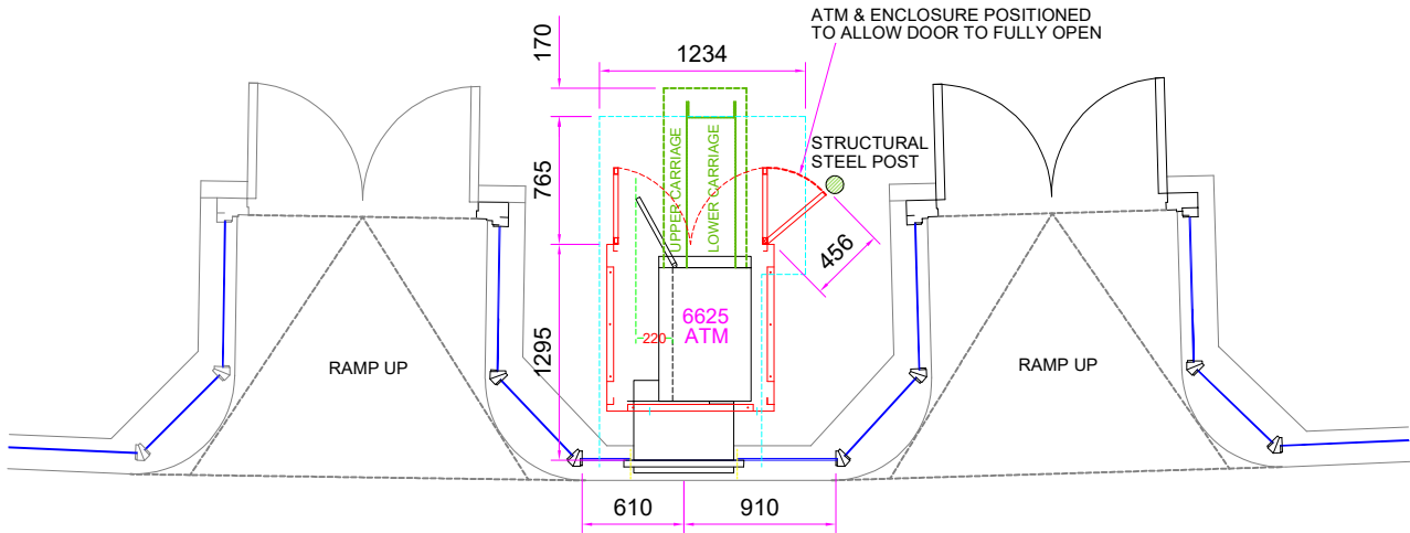
PROPOSED (PART) PLAN
