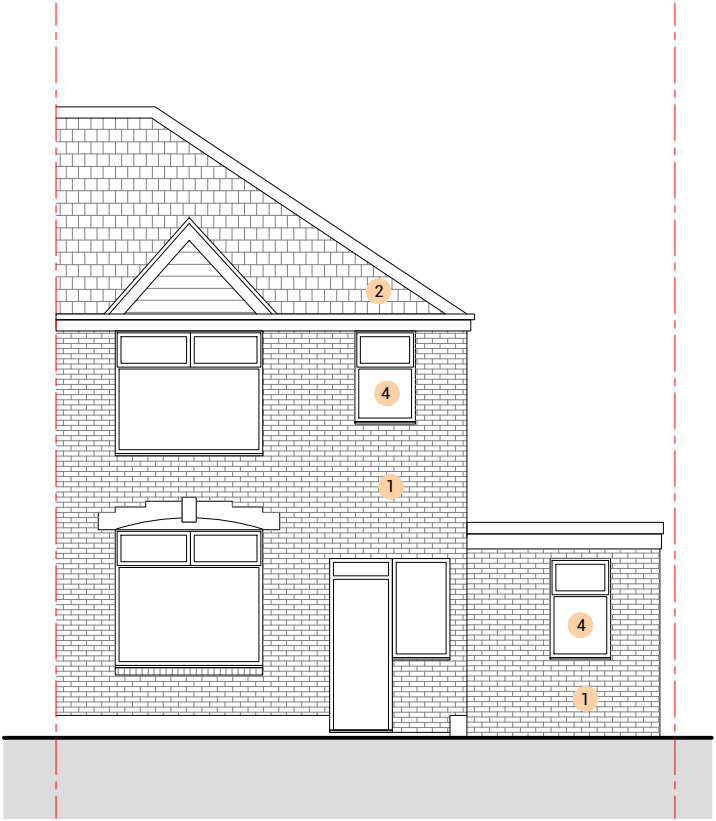
PROPOSED FRONT ELEVATION 1:100 @ A3 0m 1m 3m 5m Key 1 Brickworks to match existing 2 Roof tiles to match existing 3 PVC Window to match existing 4 PVC Window to match existing (Obscure Glazing) 5 Glazed Bifold Door 6 Roof Lantern
