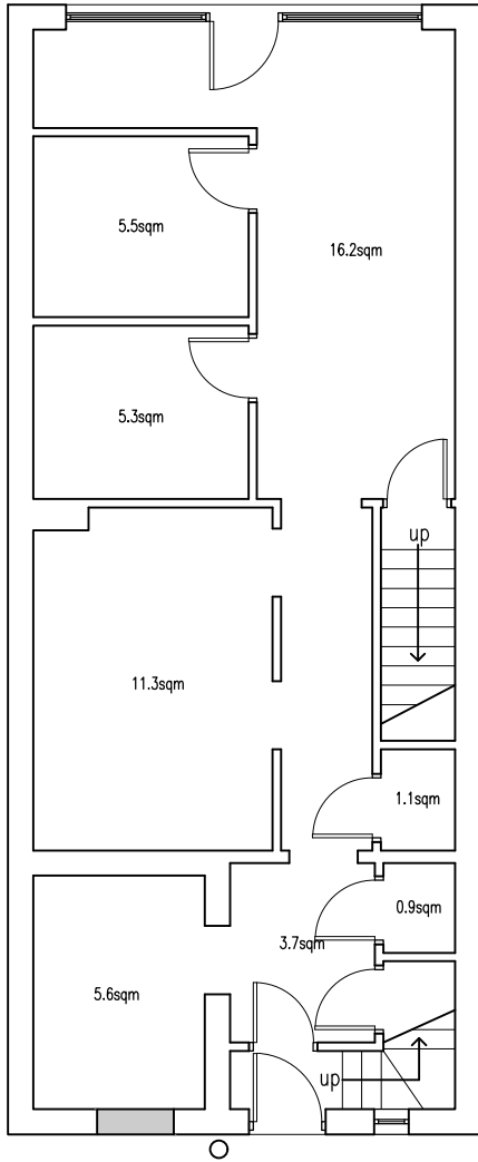
EXISTING GROUND FLOOR PLAN 1:100 @ A3
