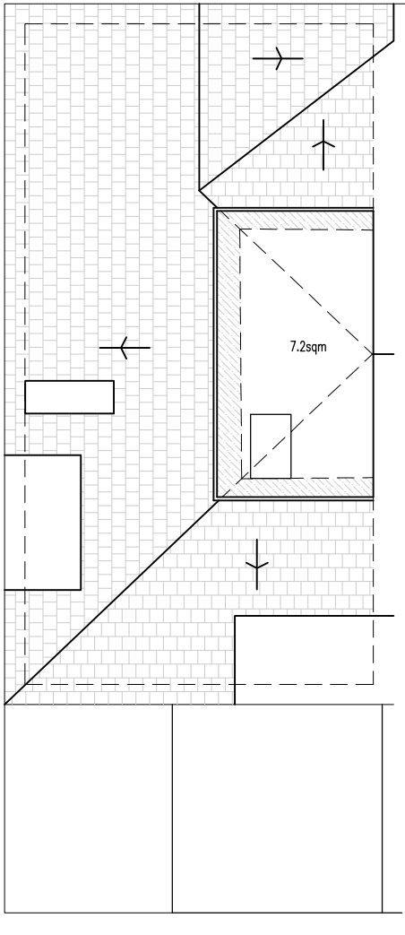
EXISTING ROOF/LOFT FLOOR PLAN 1:100 @ A3
