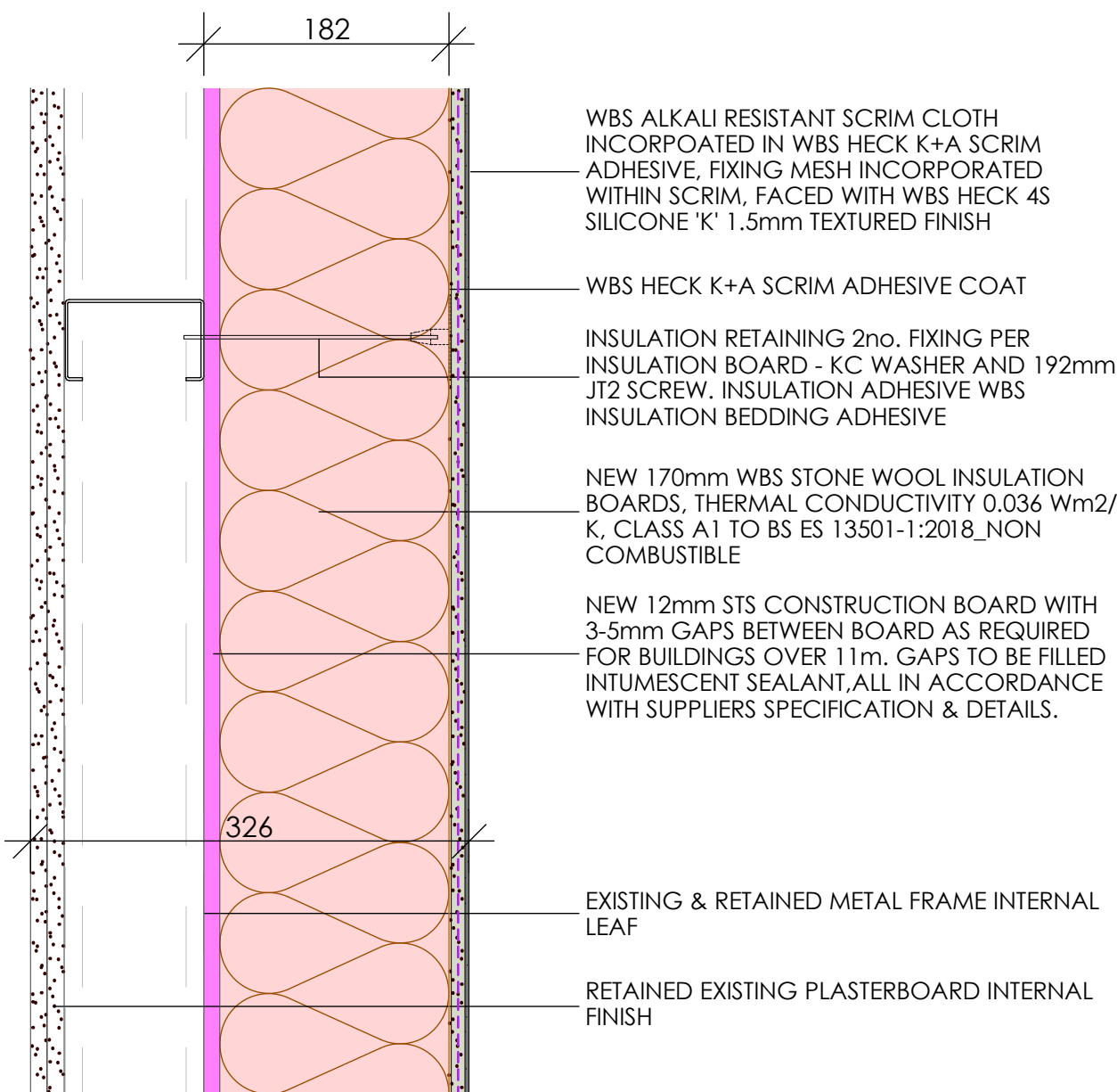
PROPOSED WALL TYPE EW02 RENDER_SFS INNER LEAF
