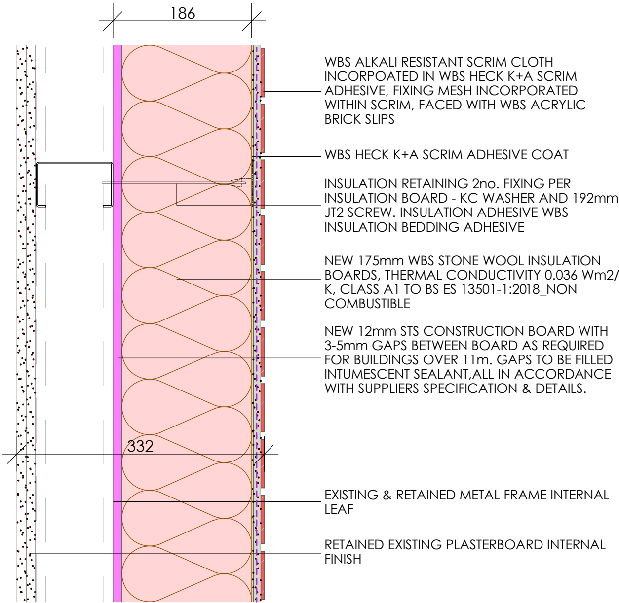
PROPOSED WALL TYPE EW01 BRICK_SLIPS_SFS INNER LEAF
