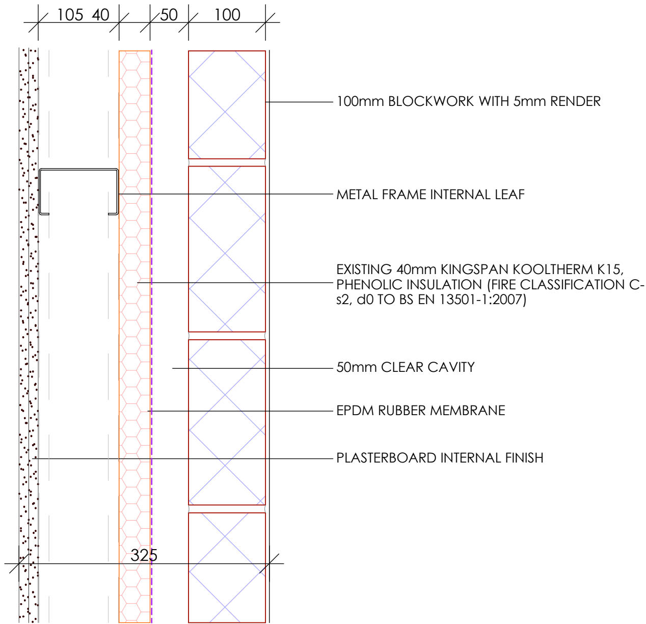
EXISTING WALL TYPE EW02 RENDER_PHENOLIC_SFS INNER LEAF
