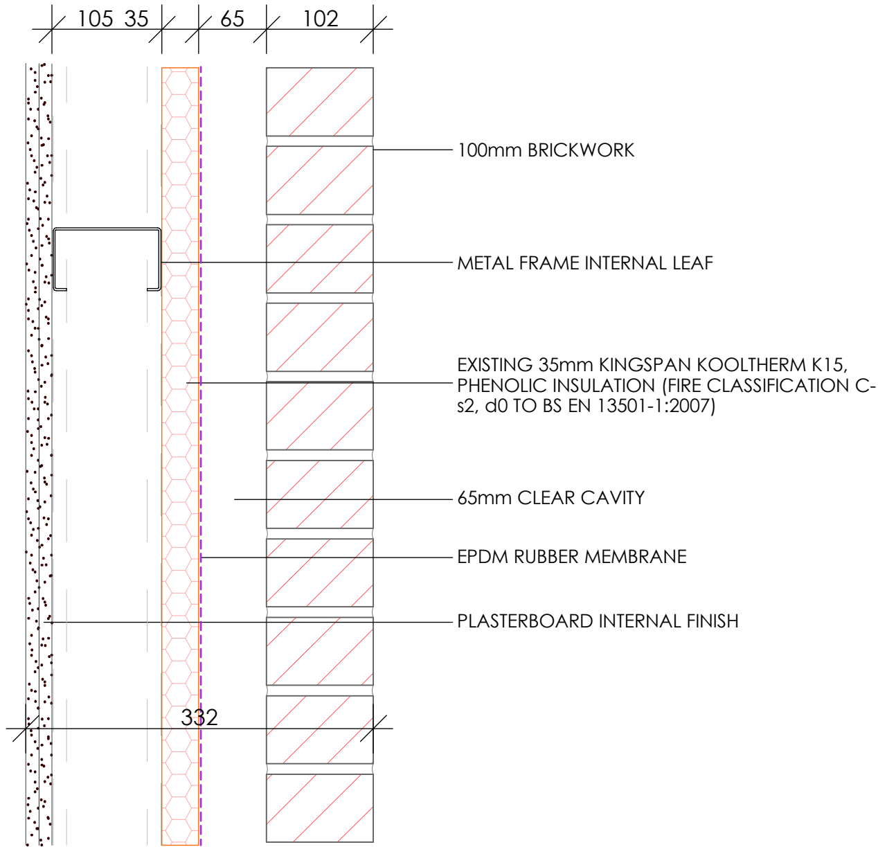
EXISTING WALL TYPE EW01 BRICK_PHENOLIC_SFS INNER LEAF
