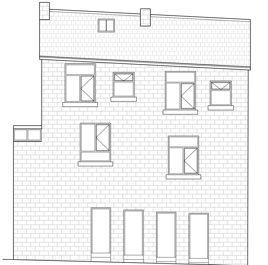
EXISTING REAR ELEVATION 1:100 @ A3
