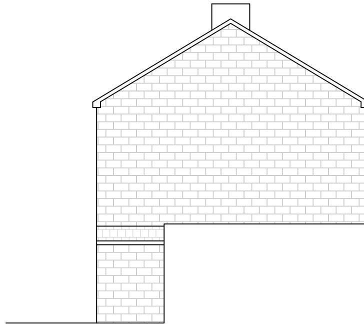
EXISTING SIDE ELEVATION 1:100 @ A3
