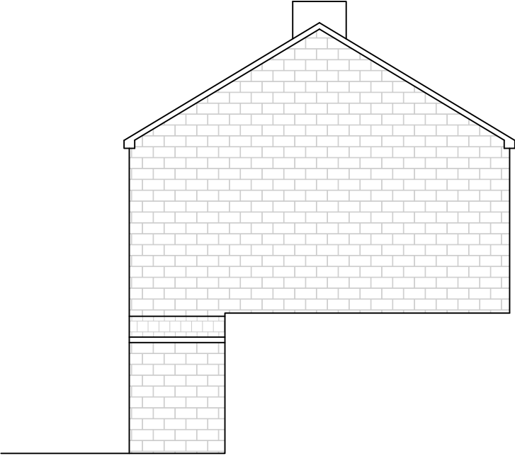
PROPOSED SIDE ELEVATION 1:100 @ A3
