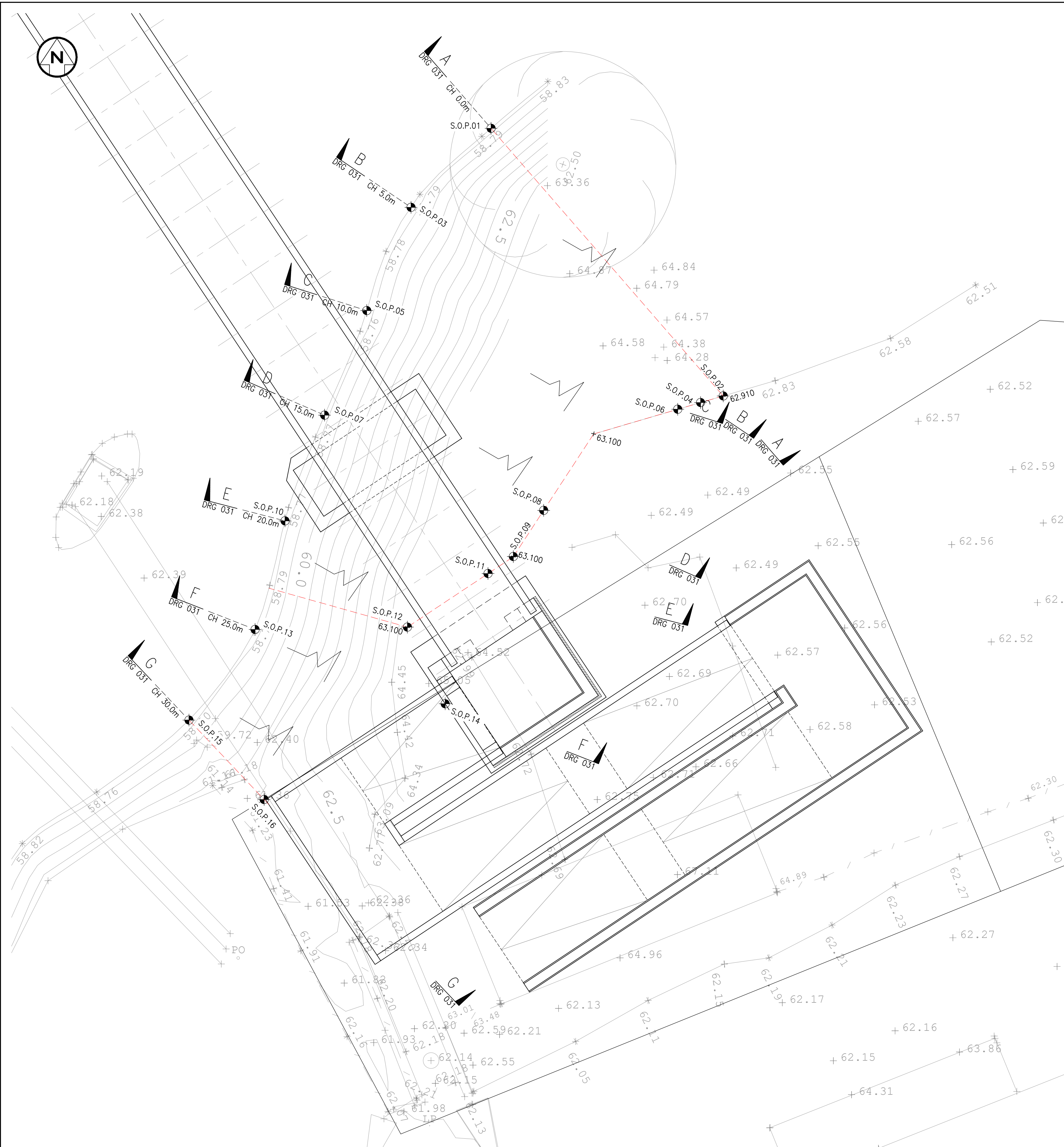
PROPOSED SOUTH APPROACH PLAN Scale 1:100
