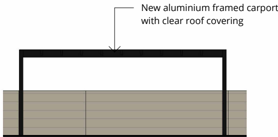
8 Carport - Proposed Rear Side Elevation 1 : 100
