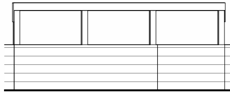
4 Carport - Existing Rear Side Elevation 1 : 100
