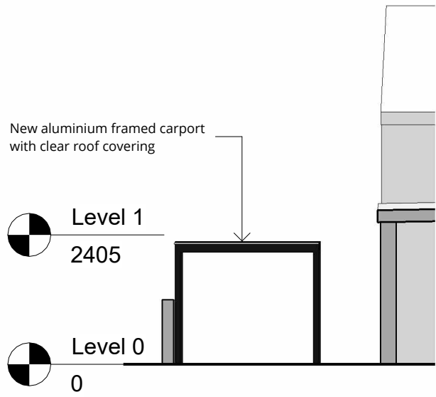
7 Carport - Proposed Rear Elevation 1 : 100
