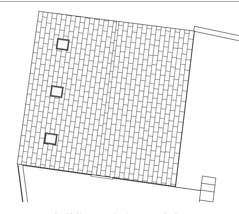
3 Outbuilding - Existing Roof Plan 1 : 100
