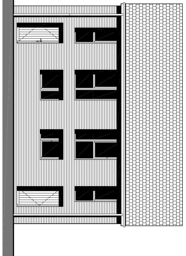
Rear Elevation Plots 15-18
