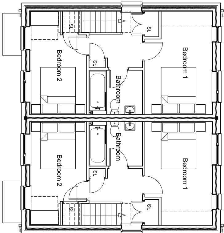
First Floor Plan Plots 15-18
