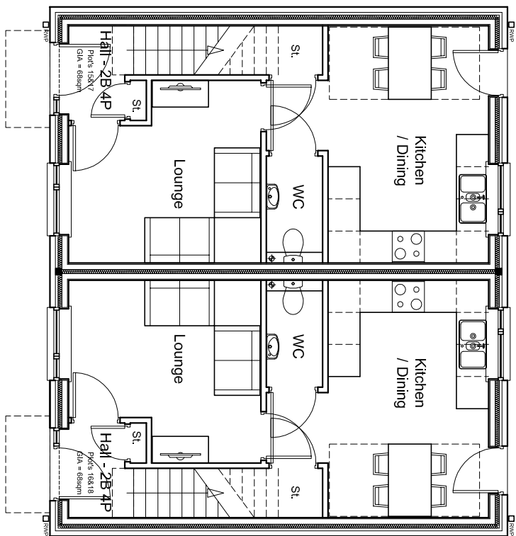
Ground Floor Plan Plots 15-18
