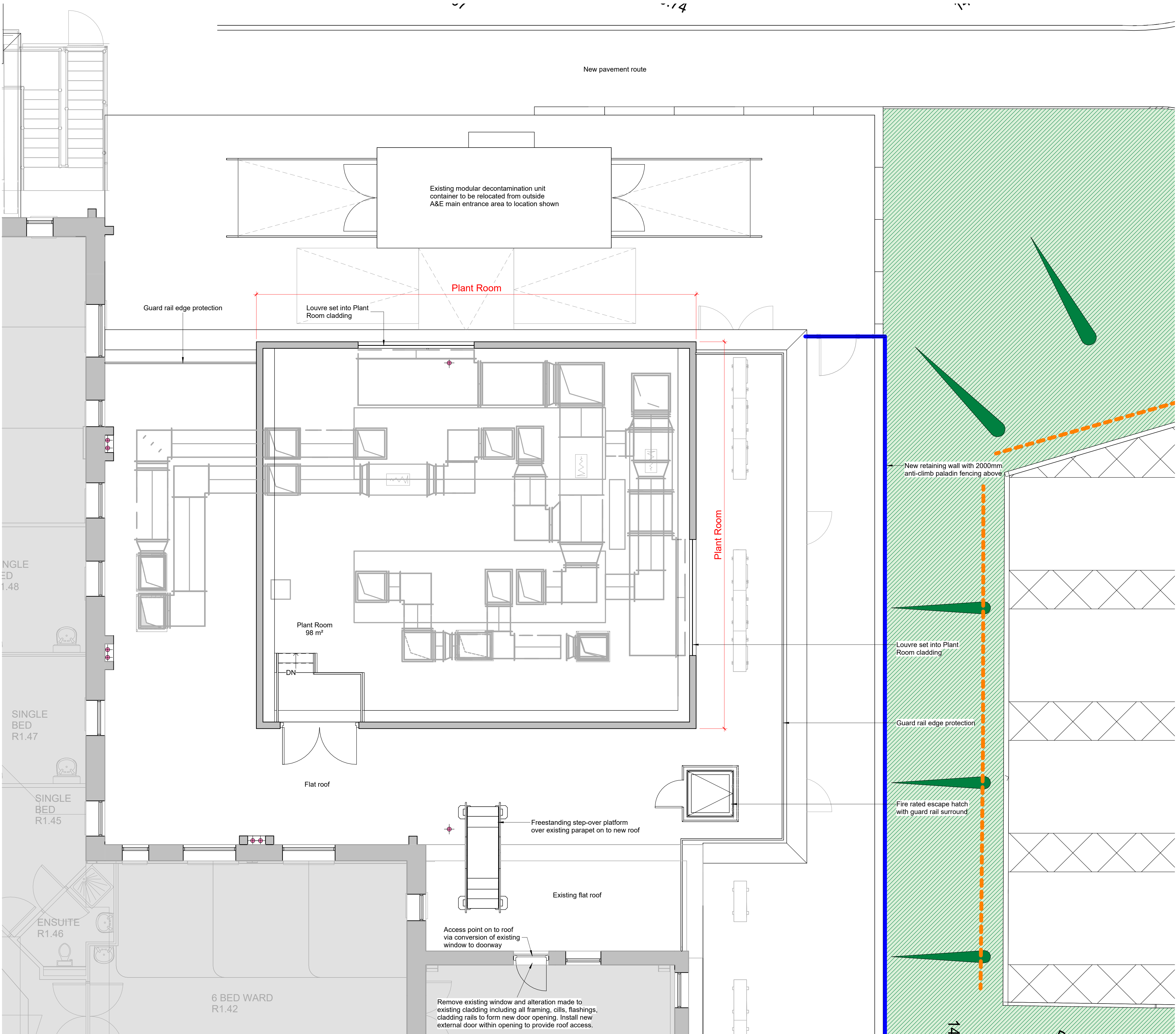
1 Plant Room 1 : 50
