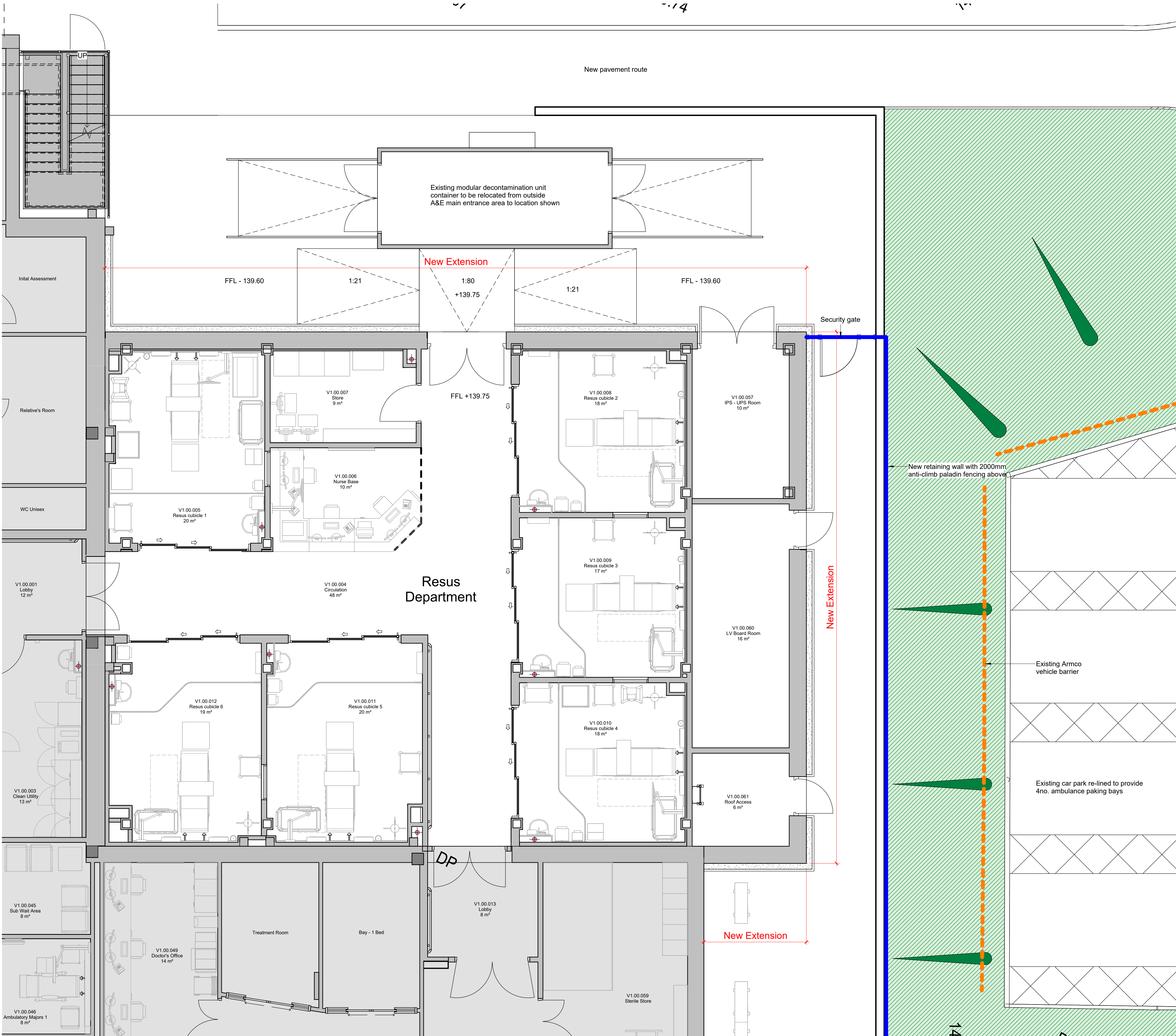
1 Proposed GA Plan 1 : 50
