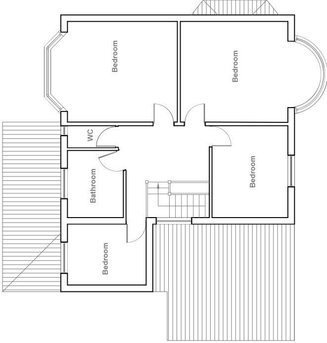
EXISTING FIRST FLOOR PLAN 1:100 @ A3
