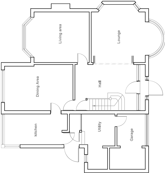
EXISTING GROUND FLOOR PLAN 1:100 @ A3
