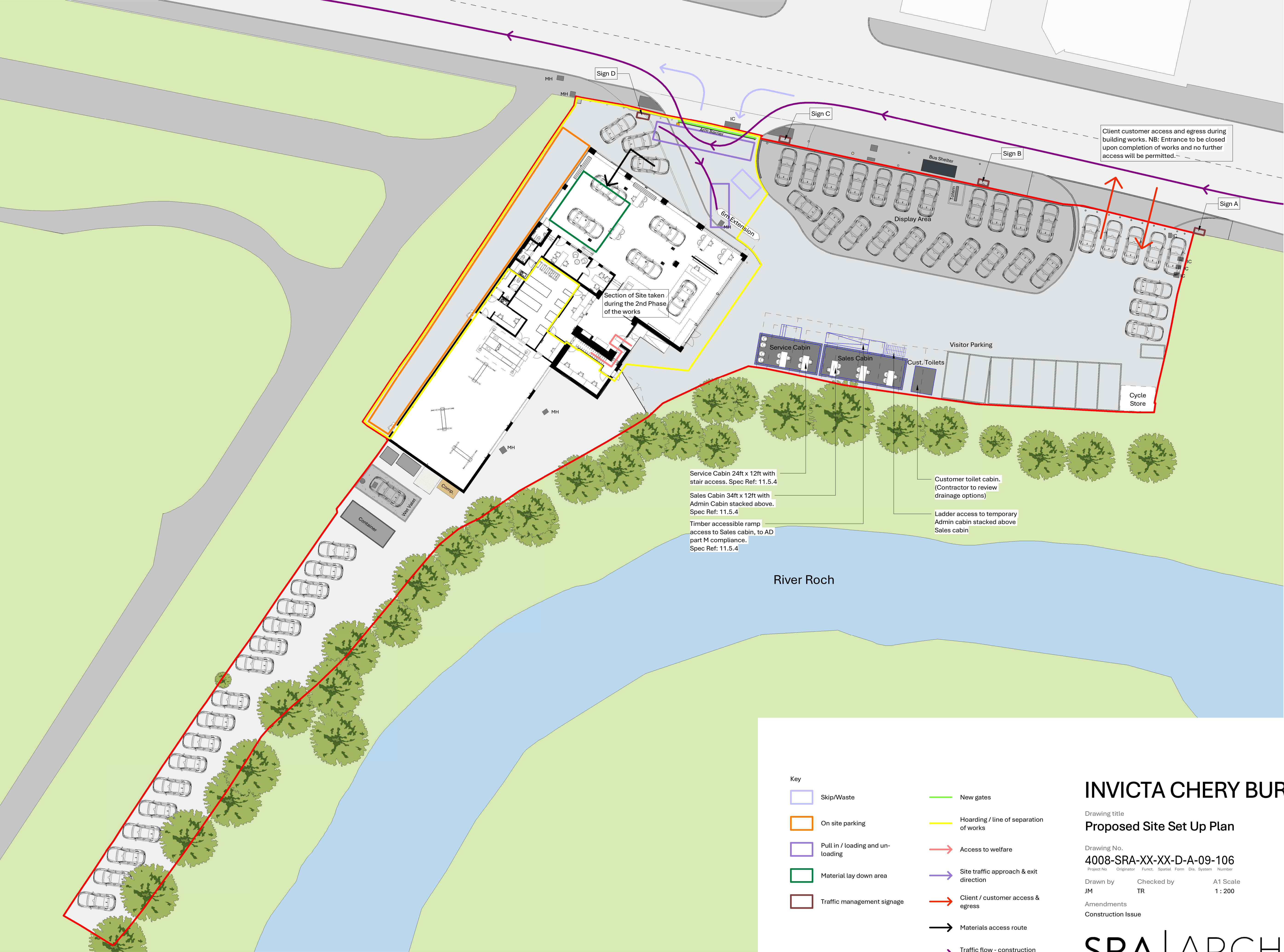
1 - 09 - Proposed Site Set Up Plan 1 : 200
