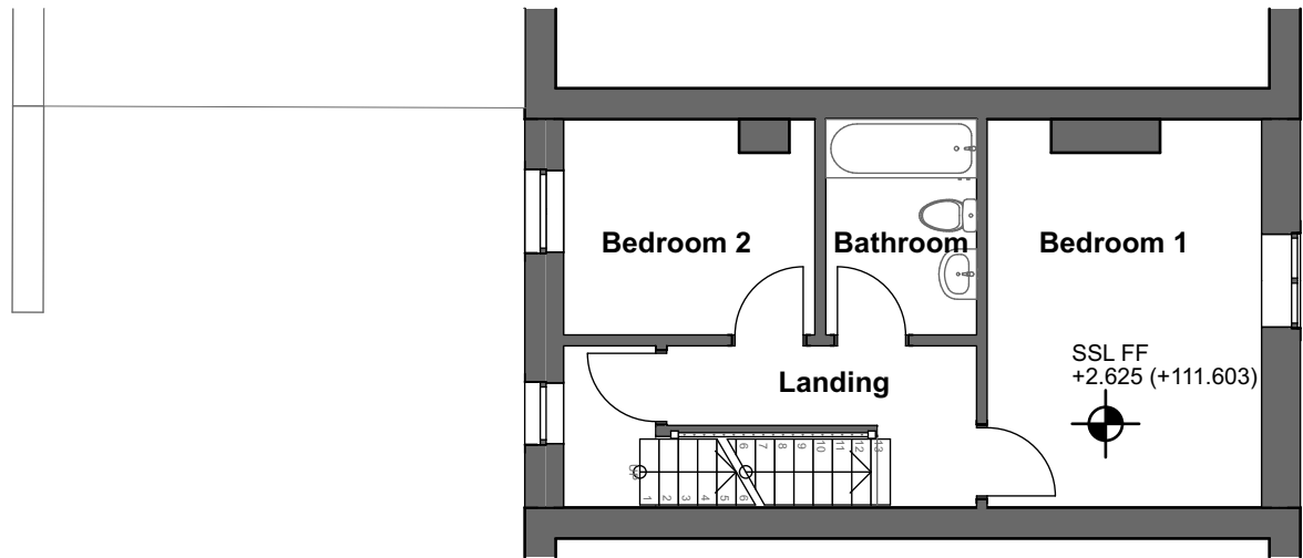
3 01-First Floor 1:100
