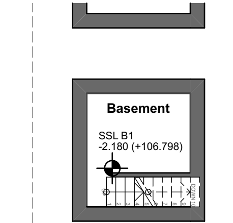
1 B1-Basement 1:100
