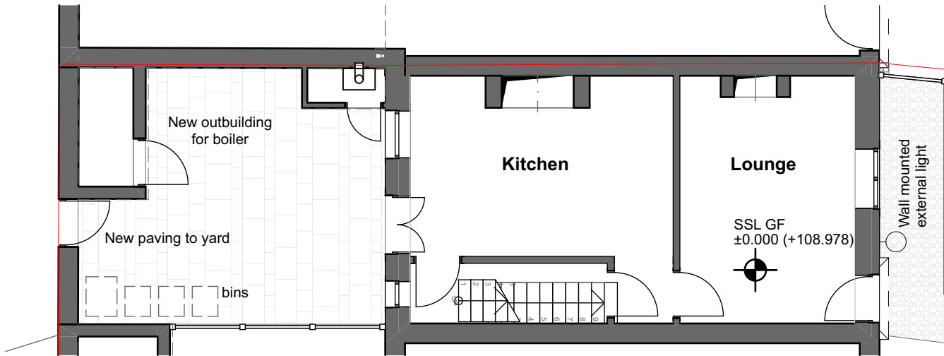
2 GF-Ground Floor 1:100
