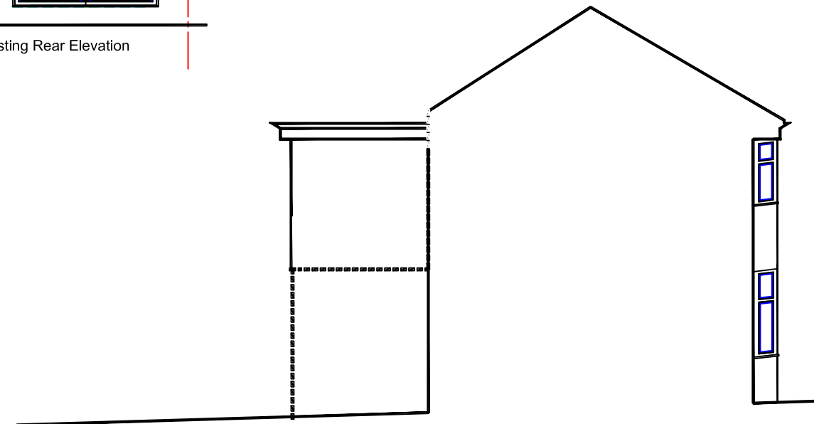
Existing Party Wall Elevation
