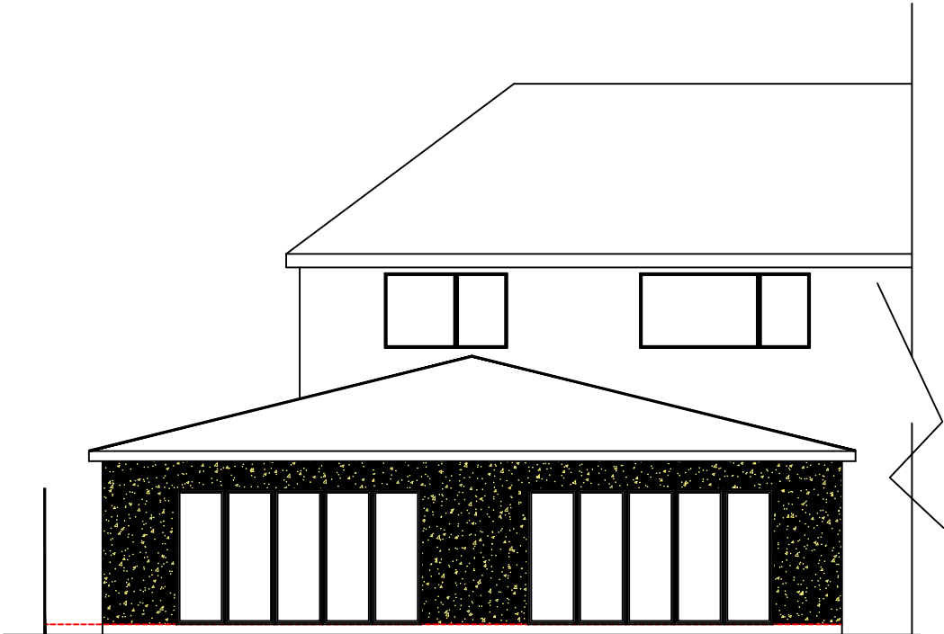
Rear Elevation
