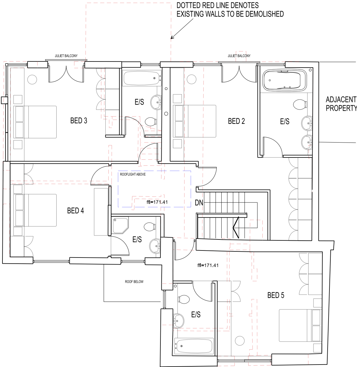
FIRST FLOOR
