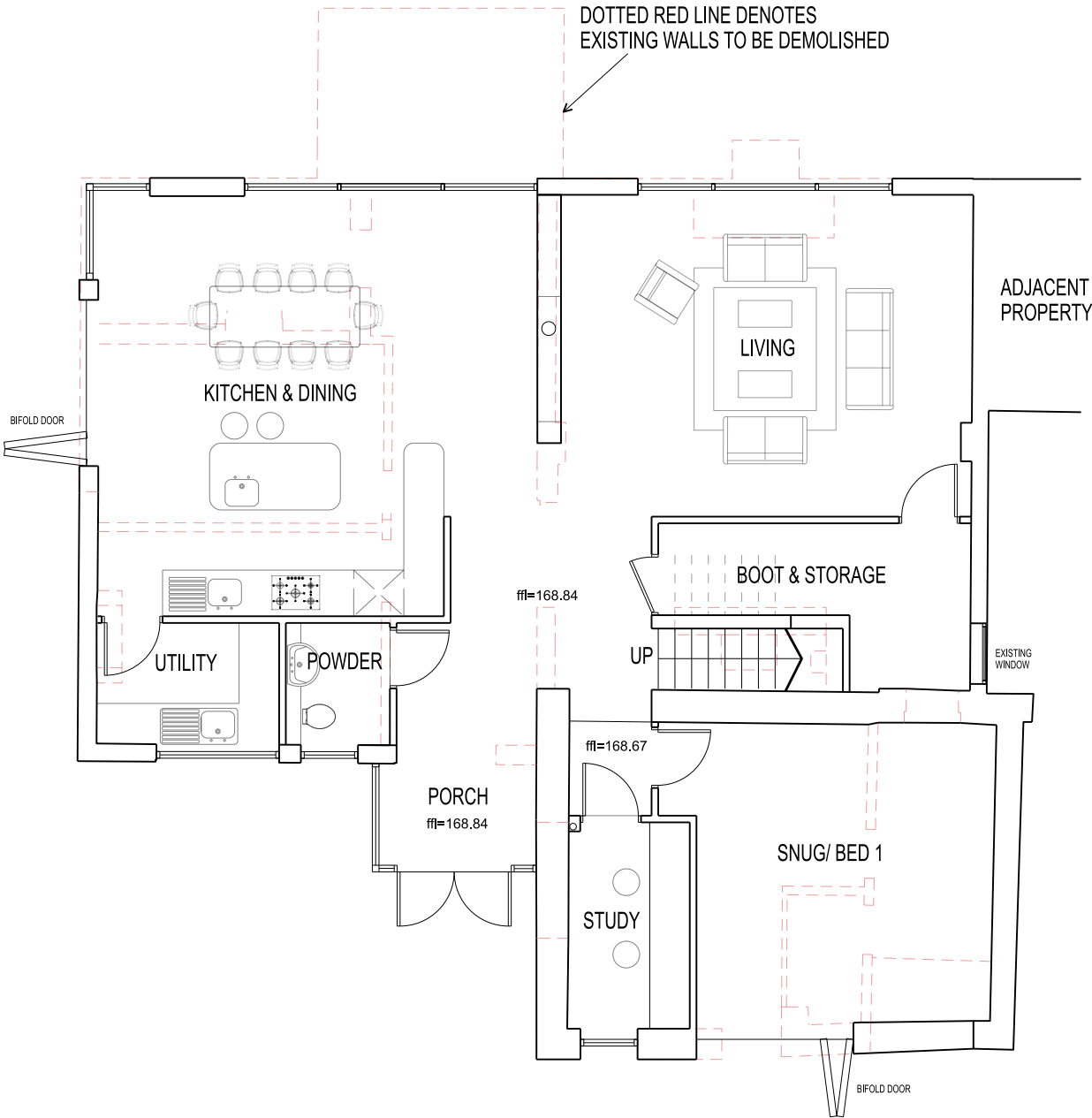
GROUND FLOOR
