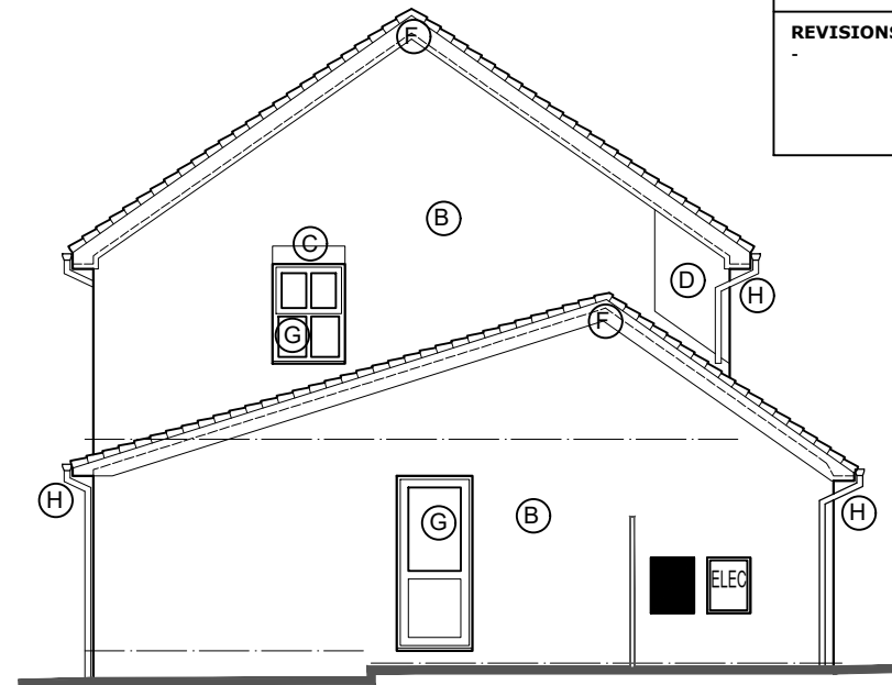
SIDE ELEVATION
